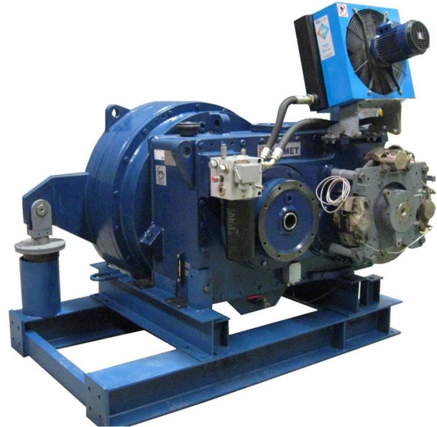
Final Assembly Including Brake Element
